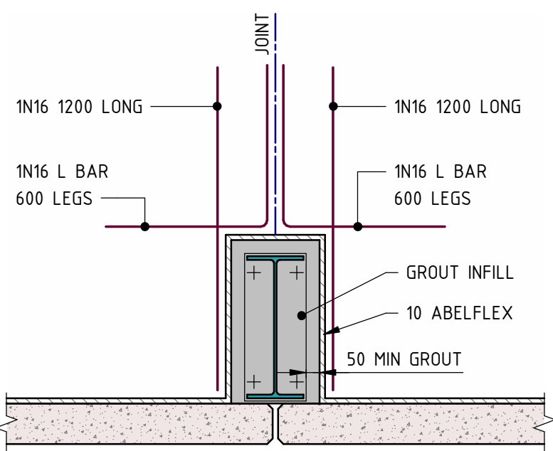
EDGE UB/UC COLUMN AT JOINT ENCAPSULATE COLUMN AND BASE PLATE IN 50 MIN NON SHRINK GROUT
