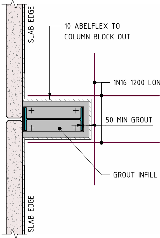
EDGE UB/UC COLUMN ENCAPSULATE COLUMN AND BASE PLATE IN 50 MIN NON SHRINK GROUT
