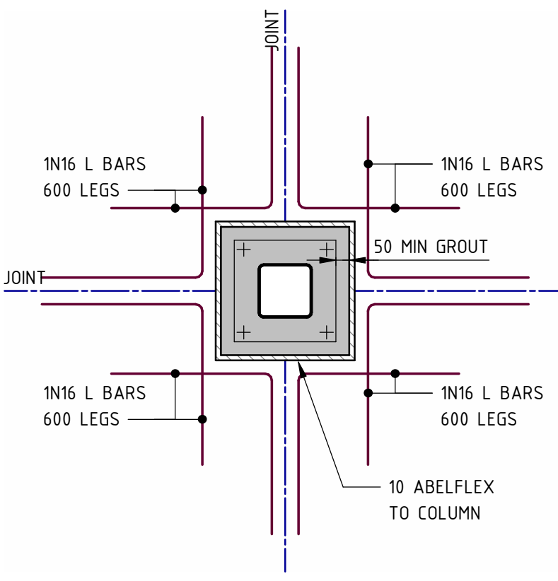
INTERNAL SHS COLUMN JOINT INTERSECTION ENCAPSULATE COLUMN AND BASE PLATE IN 50 MIN NON SHRINK GROUT
