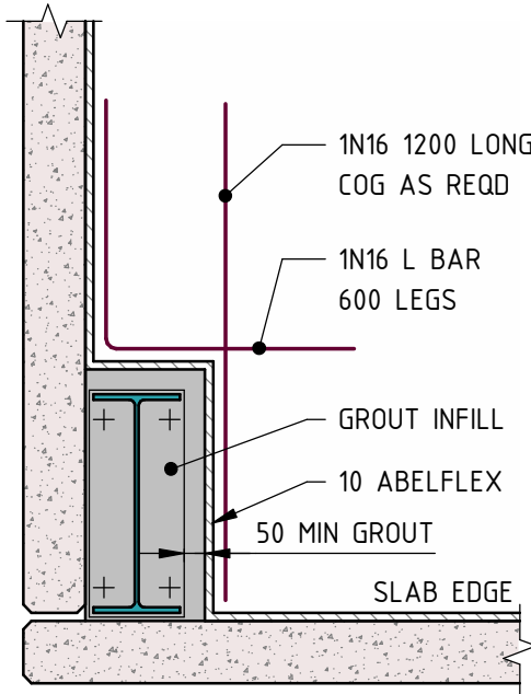
CORNER UB/UC COLUMN ENCAPSULATE COLUMN AND BASE PLATE IN 50 MIN NON SHRINK GROUT
