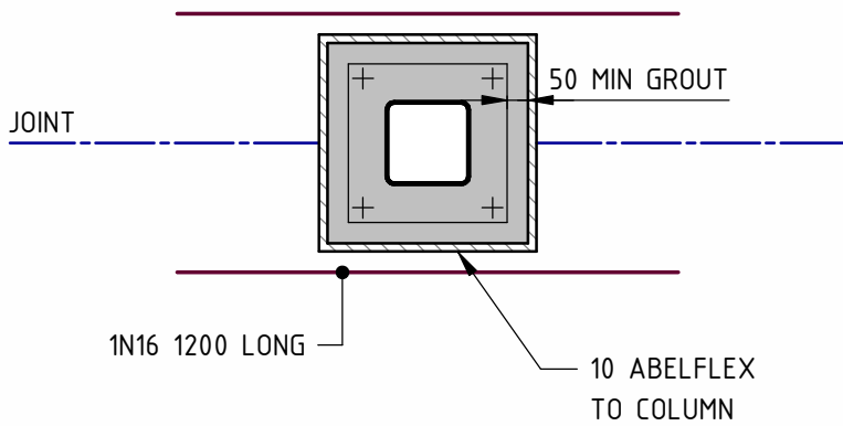
INTERNAL SHS COLUMN JOINT 'T' INTERSECTION ENCAPSULATE COLUMN AND BASE PLATE IN 50 MIN NON SHRINK GROUT
